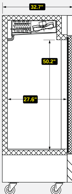
Side View
